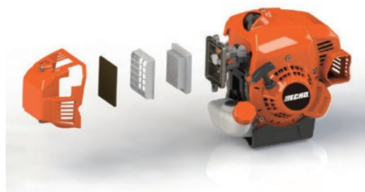
Professional two-stage air filter system provides enhanced durability
