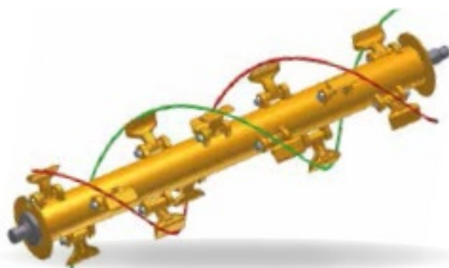
The dynamically balanced rotor has the blades situated in a spiral pattern for smooth operation.
