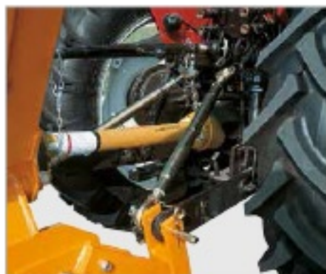
Tractor stabilizers maintain rigidity on the tractor.
