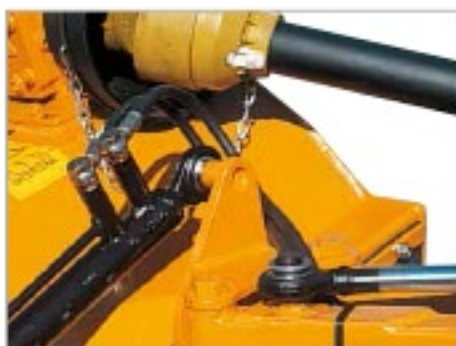
The arms rotating pivot has a self-lubricating bearing for minimal maintenance.
